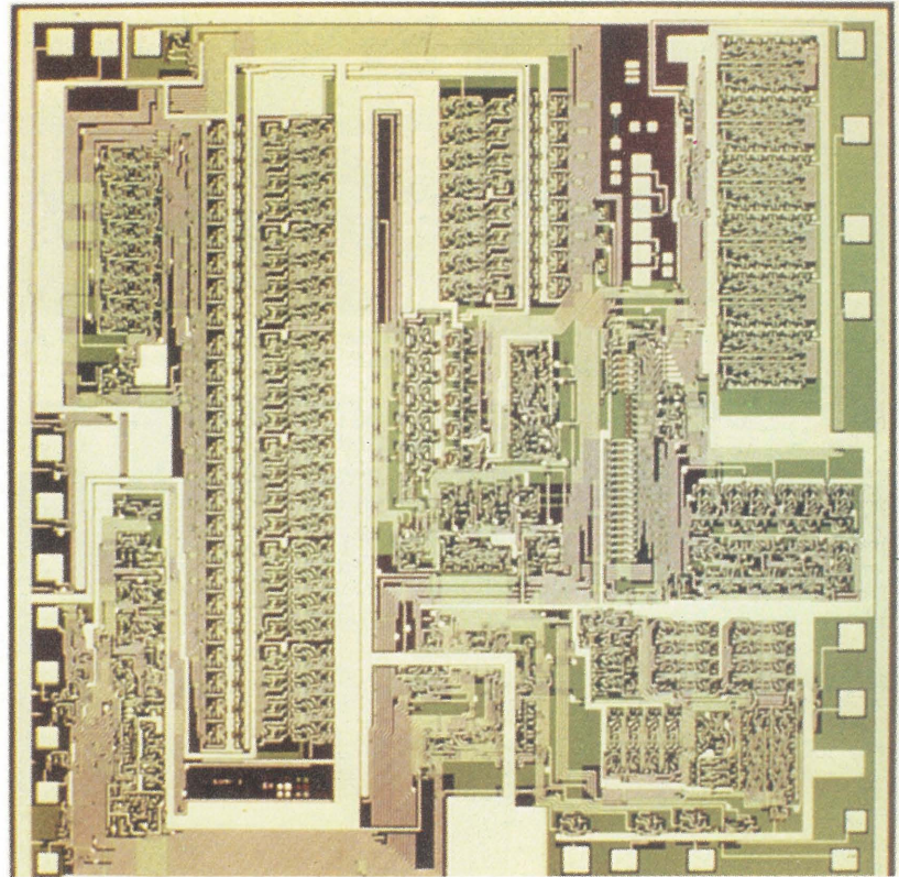
25 A chip embodying 15 different functions and measuring about 6 millimetres square designed for use in a counter.
