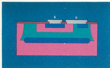
Diode
